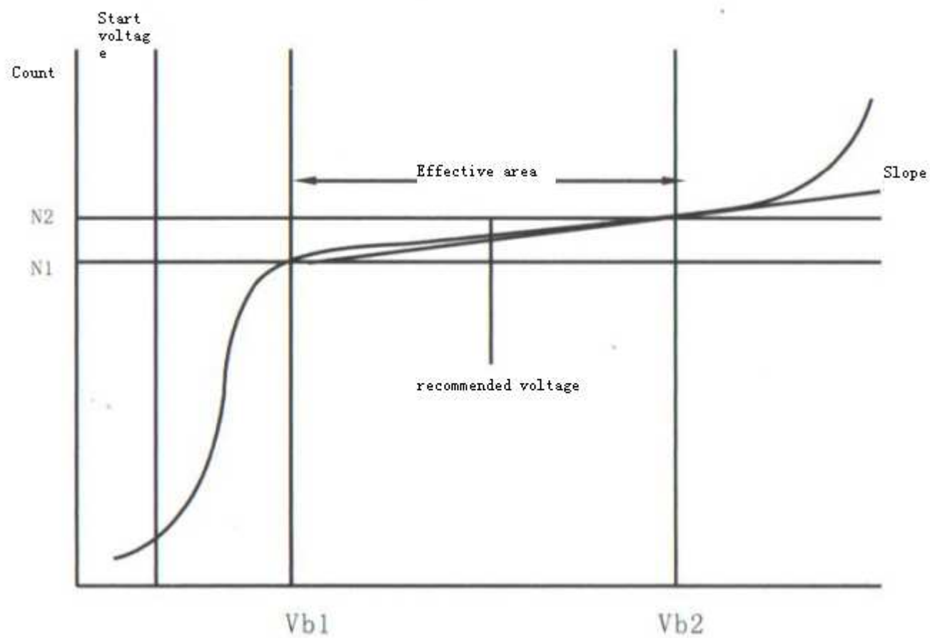
M4011 Slope specifications
