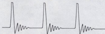
Figure 3 — Voltage Waveshape
