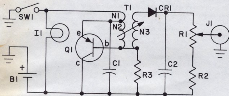
Figure 2 — Schematic
