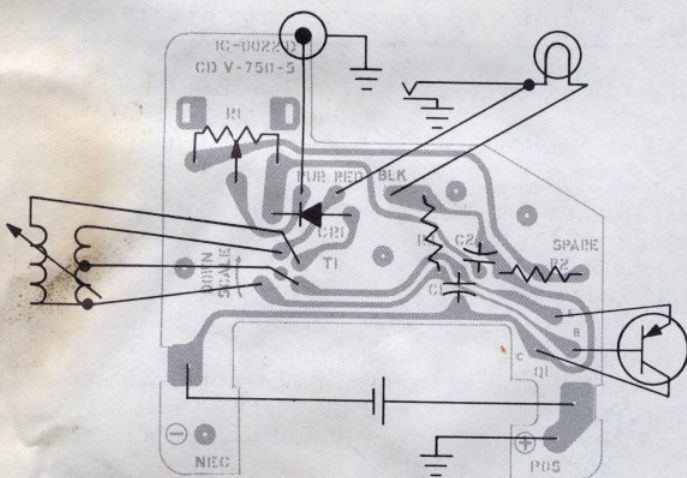
Figure 4 — Wiring Diagram
